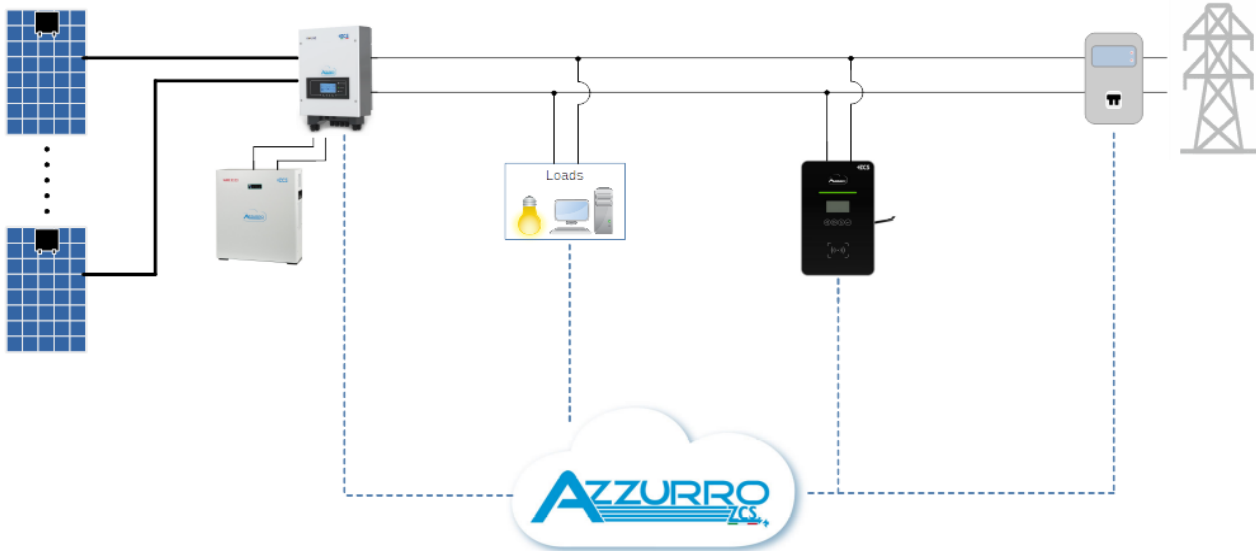
Figure 36 - Plug&Play mode
