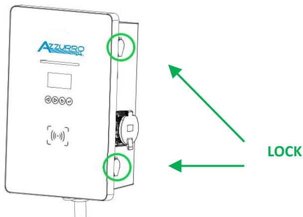
Figure 18 – Lock position
