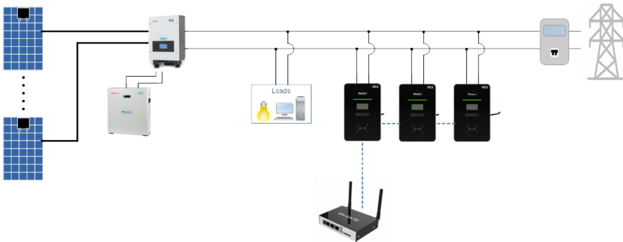
Figure 34 - Online mode
