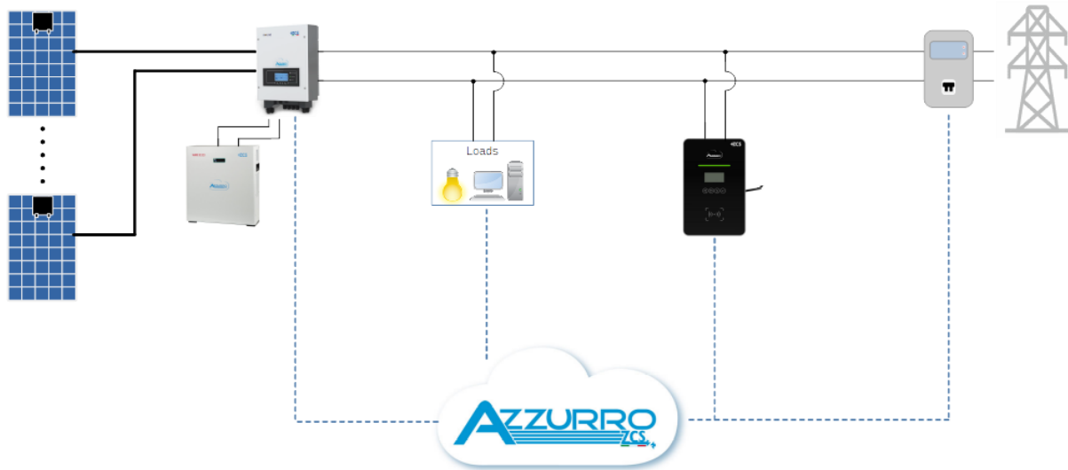
Figure 35 - Offline mode
