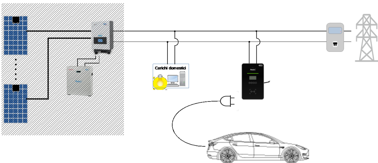
Figure 3 – Example of a charging station connected to a PV system (optional) and grid
